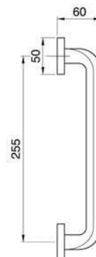
TENDER PH Maniglia Pull handle
