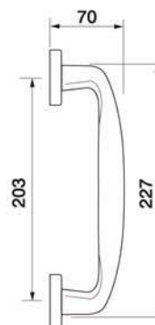
GOLF PH Maniglia Pull handle
