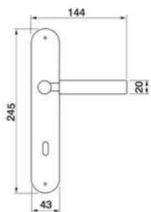
CLOUD PL Maniglia su rosetta placca Door lever handle with plate
