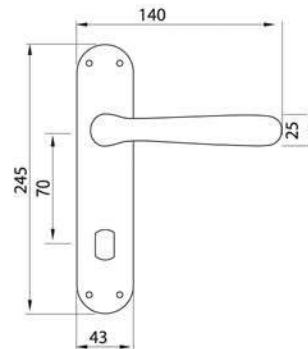
RUBINO PLB WC 70 Maniglia su WC placca Door lever handle with plate
