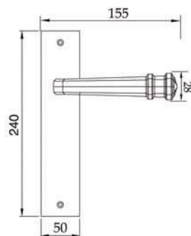
CHAMPS-ELISEES PL Maniglia su rosetta placca Door lever handle with rosette and escutcheon
