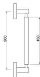
CLOUD PH Maniglia Pull handle
