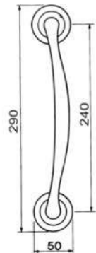
LEON PH Maniglia Pull handle
