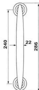
FLAMINGO PH Maniglia Pull handle
