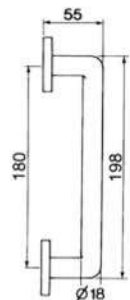
SNAKE PH Maniglia Pull handle
