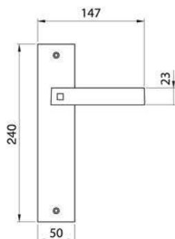
MOUNTAIN OF LIGHT PL Maniglia su rosetta placca Door lever handle with plate
