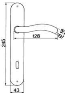
SNAKE PL Maniglia su rosetta placca Door lever handle with plate
