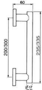
CALLA PH Maniglia Pull handle
