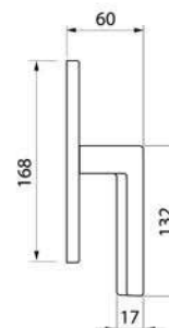
MOUNTAIN OF LIGHT W2 Maniglia per finestra Window handle
