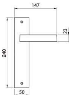
WATERFALL PL Maniglia su rosetta placca Door lever handle with plate
