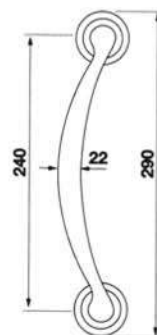
COBRA PH Maniglia Pull handle
