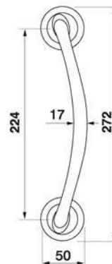
COCKATTO PH Maniglia Pull handle
