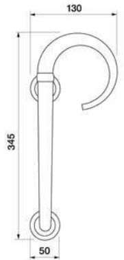
LANGOUST PH R Maniglia Pull handle right hand
