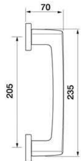
WIND PH Maniglia Pull handle
