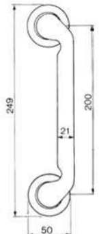
NIRVANA PH Maniglia Pull handle
